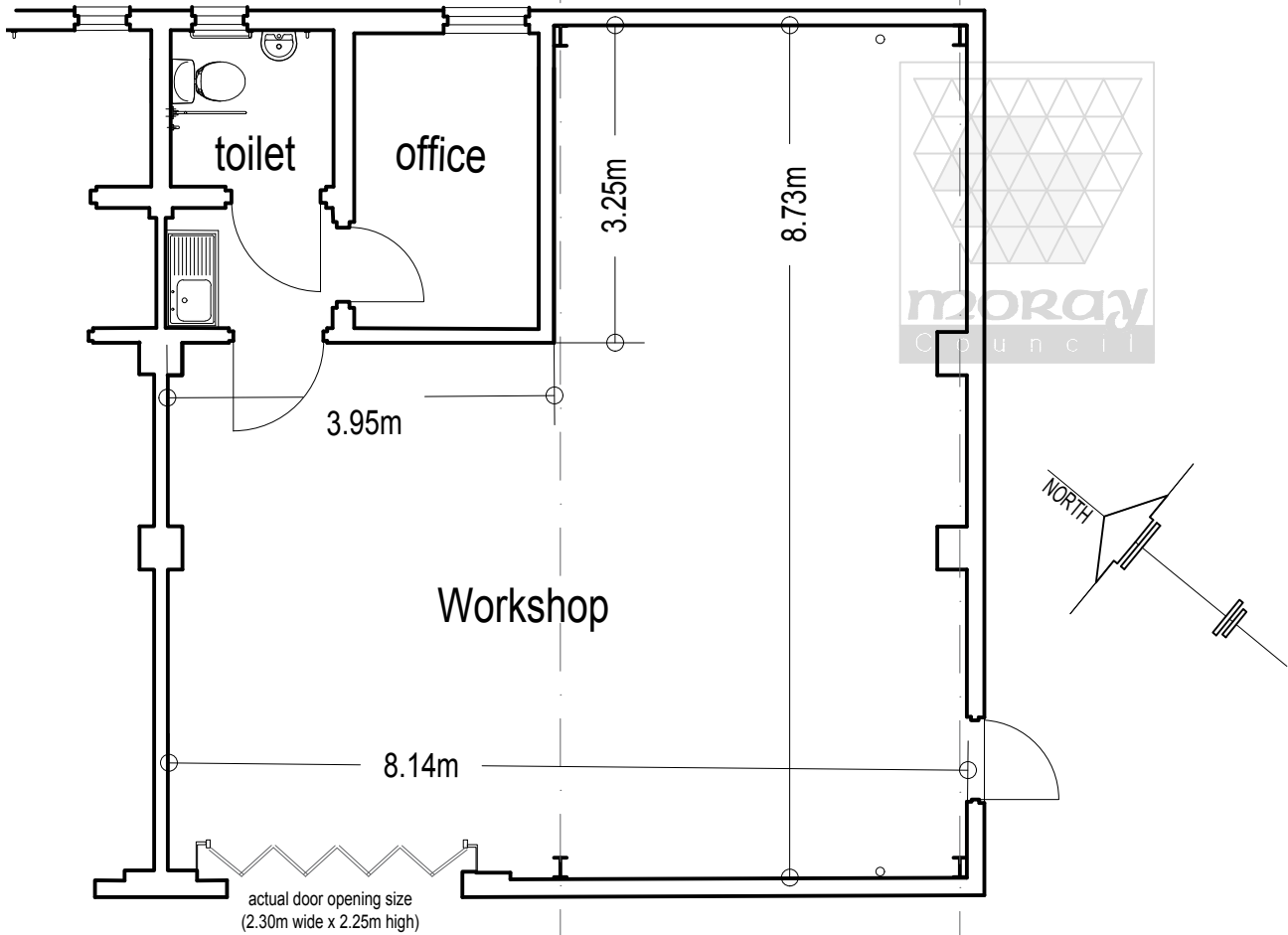
FLOOR PLAN
