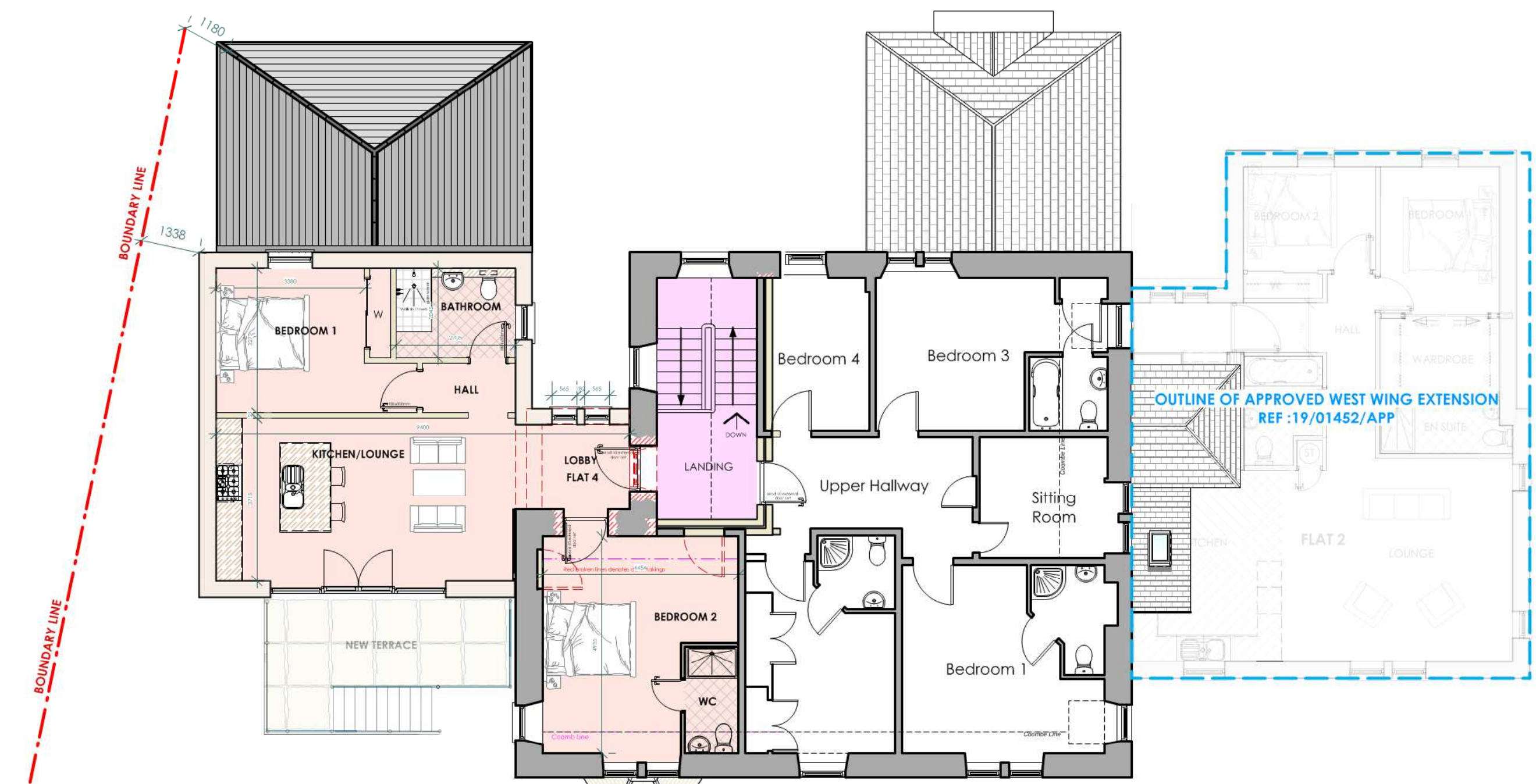
FIRST FLOOR PLAN 1:100 EXTERNAL FLOOR AREA - 63m 2
