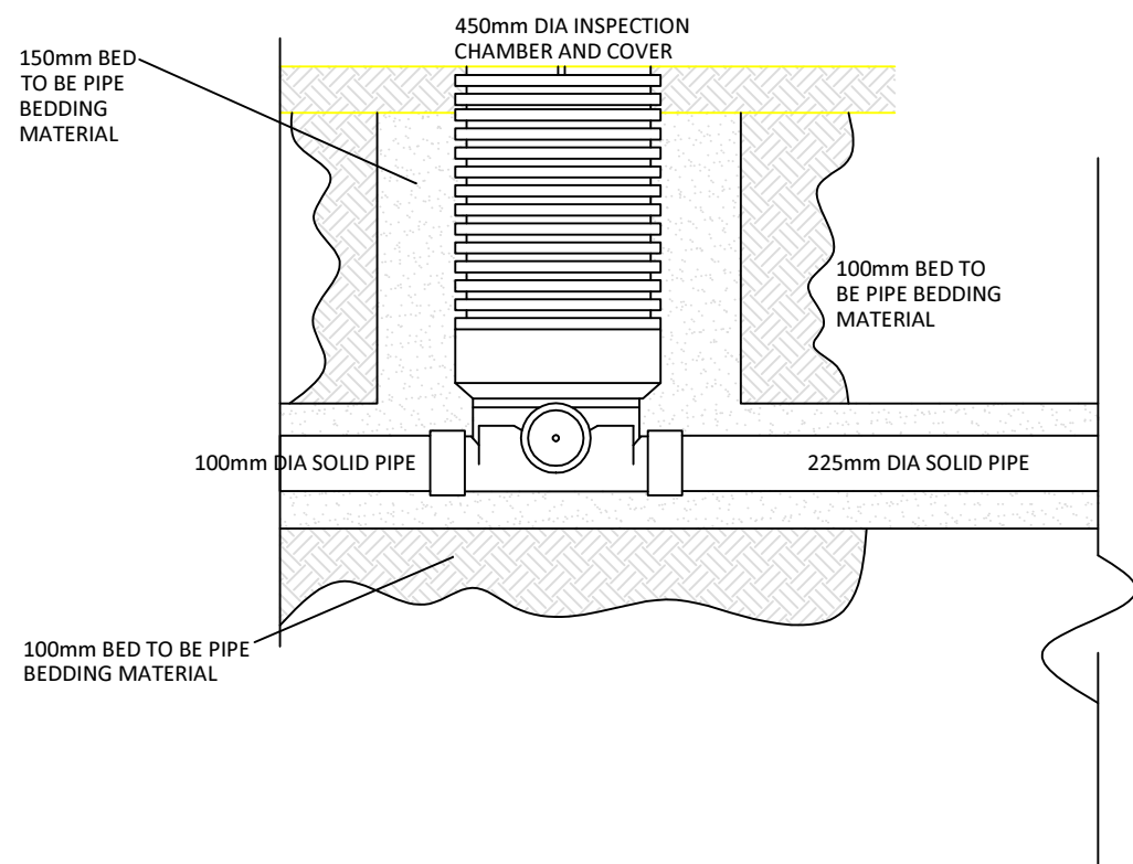
TYPICAL DETAIL THROUGH PERMEABLE PAVING WITH SOAKAWAY BEANEATH
