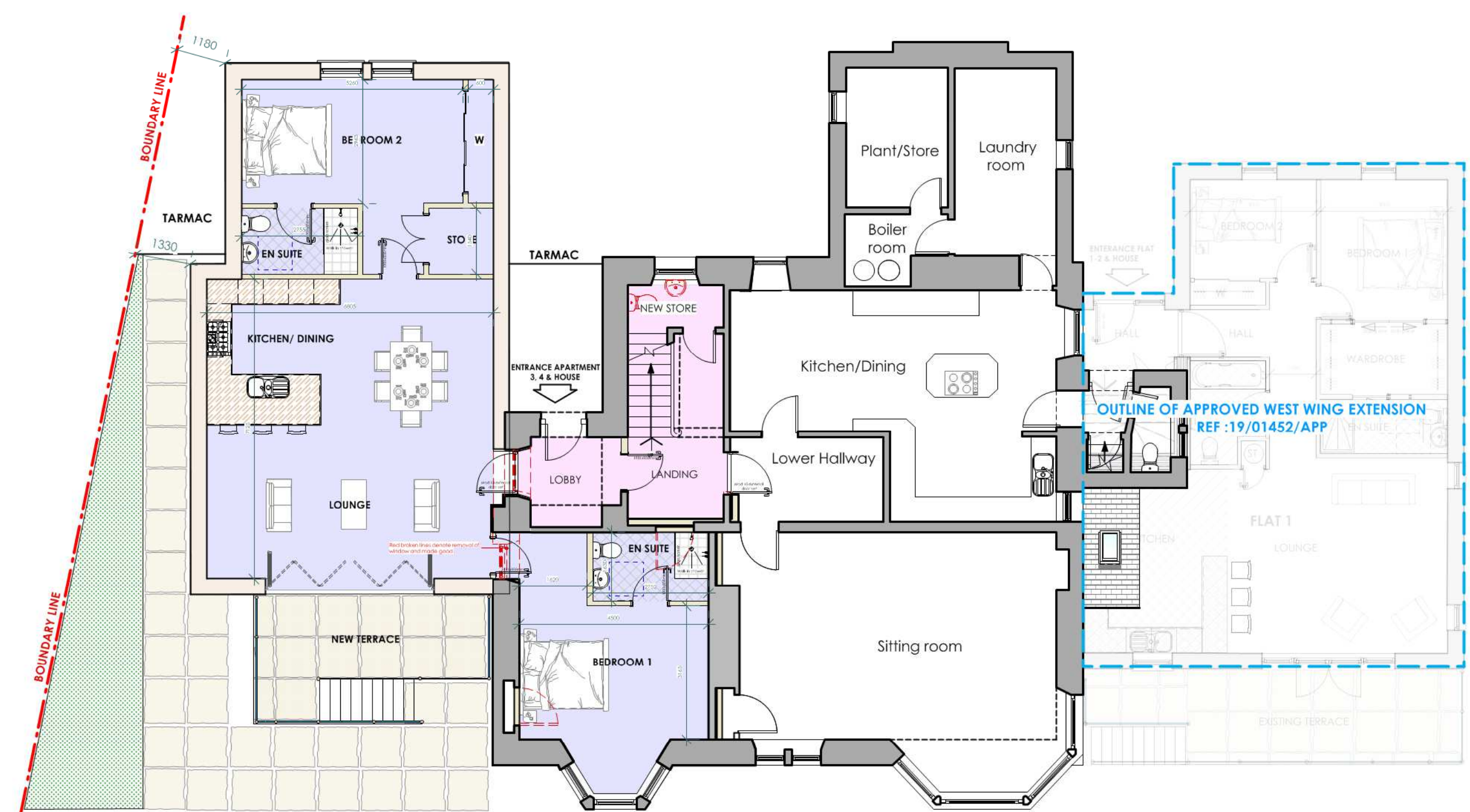
GROUND FLOOR PLAN 1:100 EXTERNAL FLOOR AREA - 91m 2
