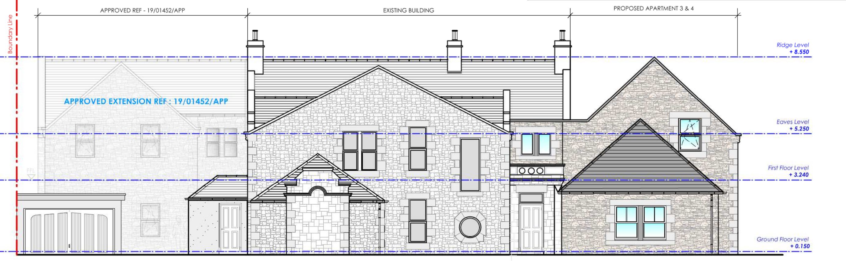
FRONT ELEVATION 1:100
