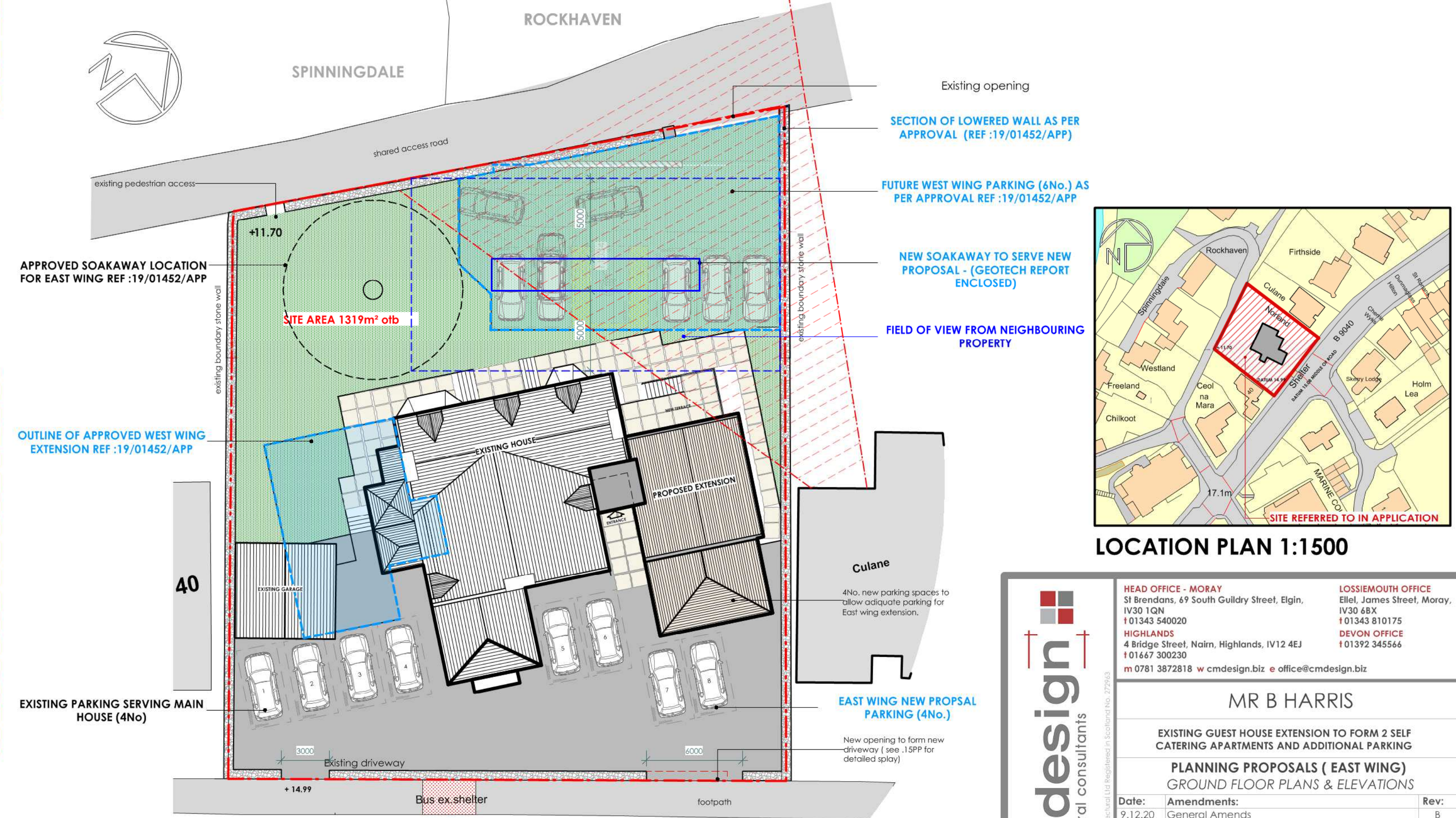
SITE & PARKING PLAN 1 : 200
