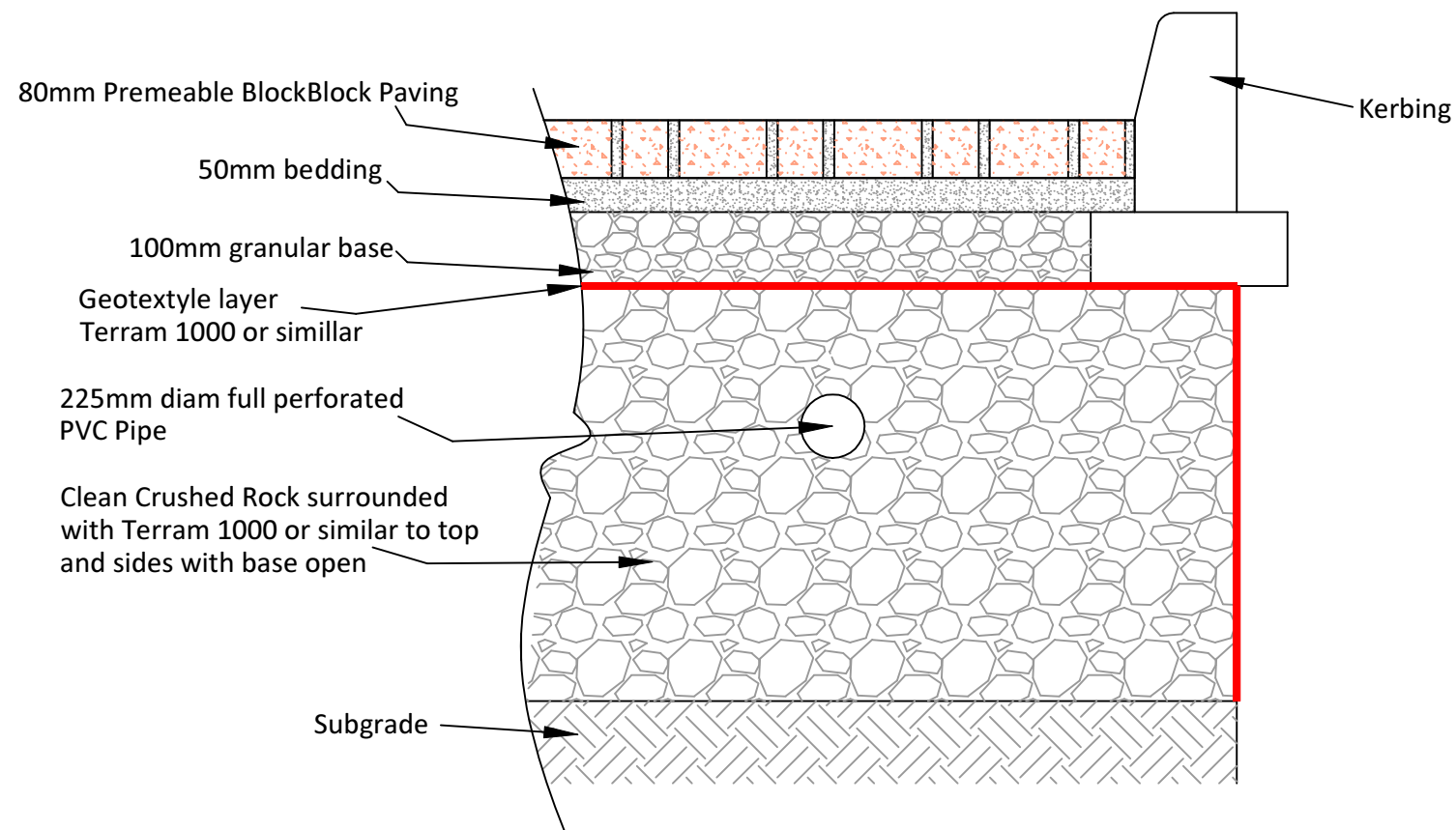
TYPICAL DETAIL THROUGH PERMEABLE PAVING WITH SOAKAWAY BEANEATH
