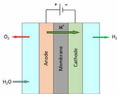
Figure 5.2: PEM Electrolysers Cell. Source: Mott MacDonald
